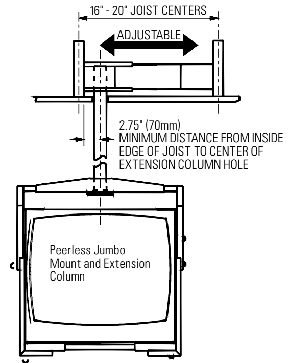
FRONT VIEW Peerless Jumbo Mount attached to Internal Joist Mount.
